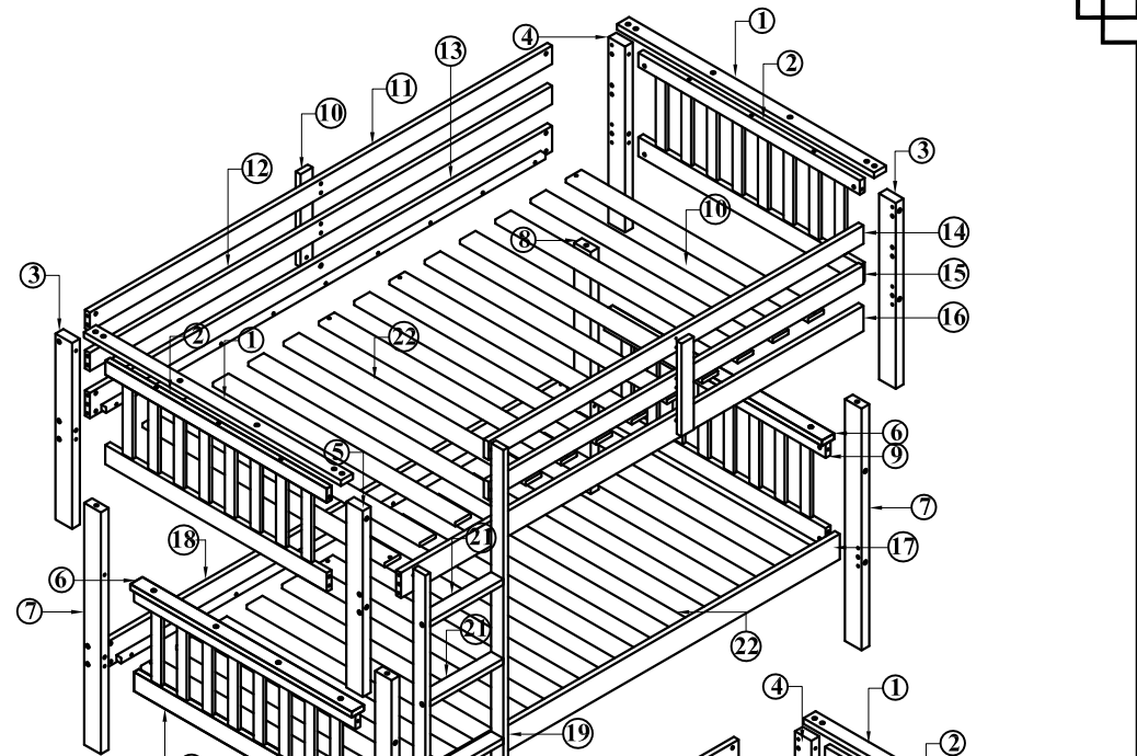
Bed Option #1 Slats - 13pcs x 2sets
